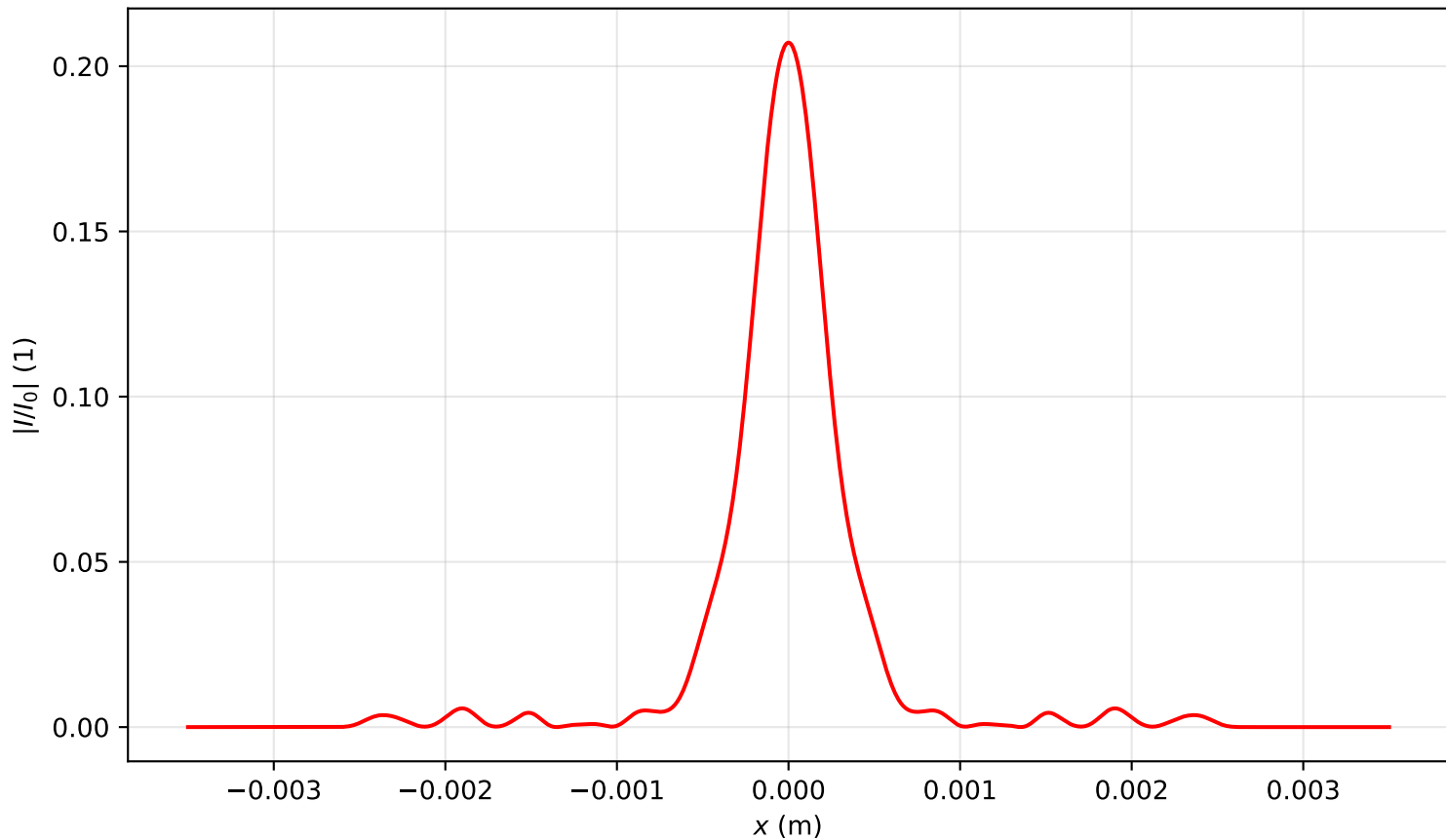
Intensity profile I(x, y = 0, z = 2.707)/I_0 , P_{in}=6.0P_{cr} , artificial time
